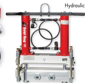
Hinged Pipe Cutters 12" (356 mm) p. 17
